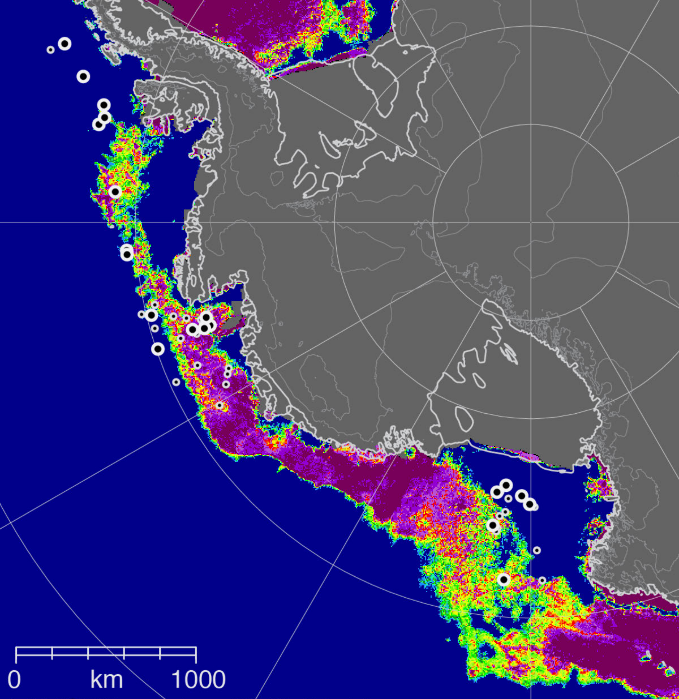
AMSR2 sea ice: 2013-01-14
