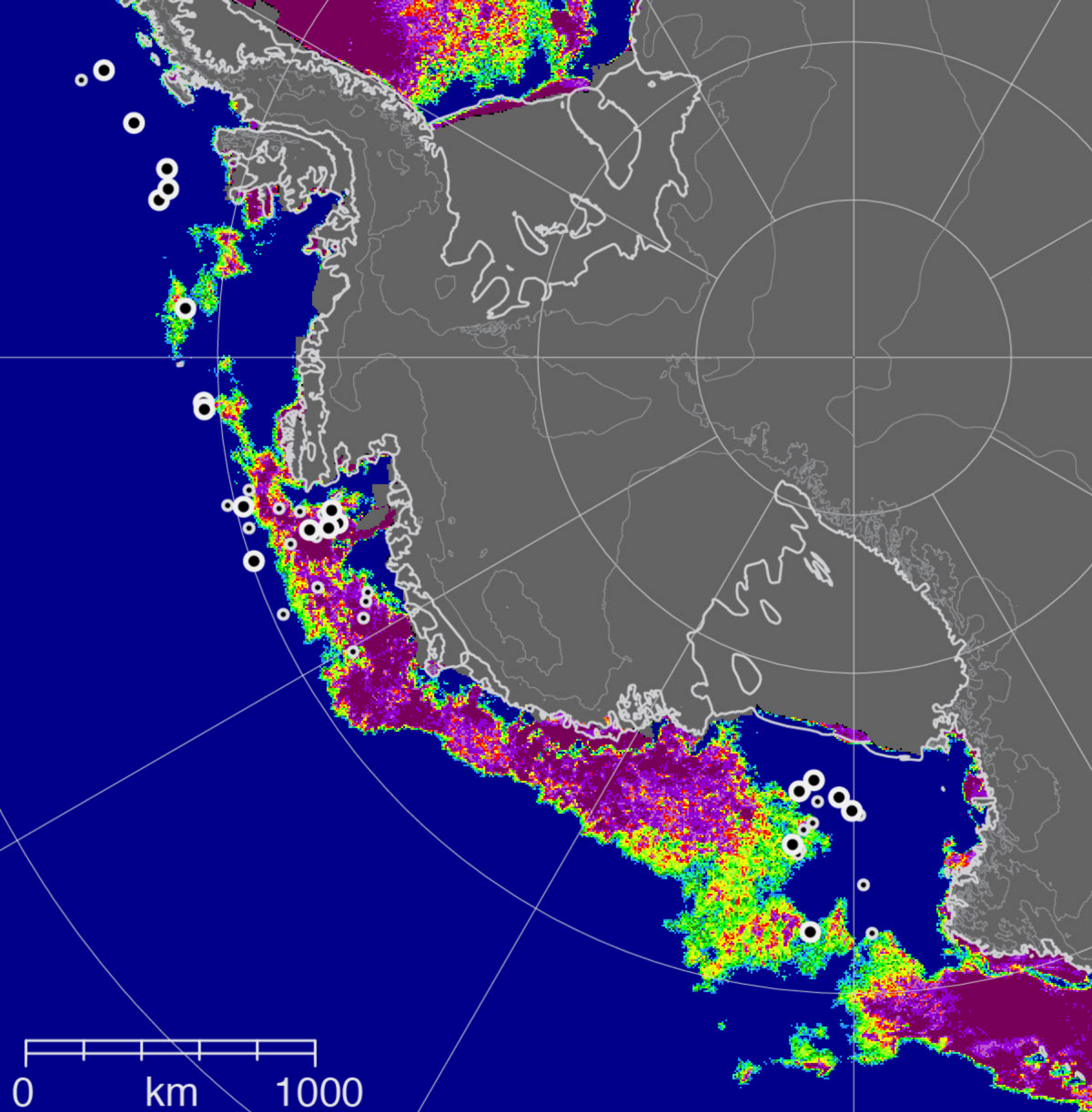
AMSR2 sea ice: 2013-01-28
