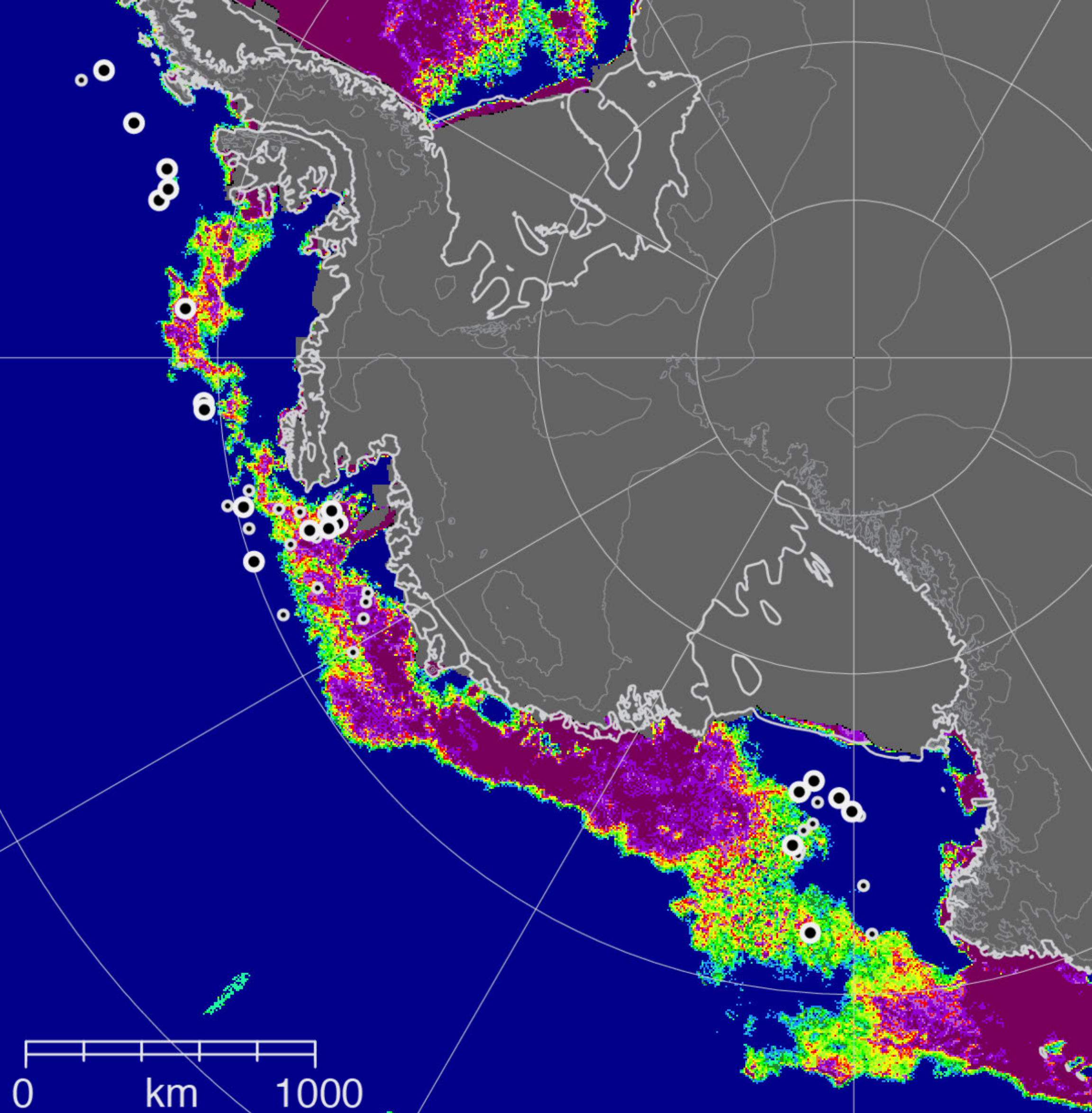
AMSR2 sea ice: 2013-01-21
