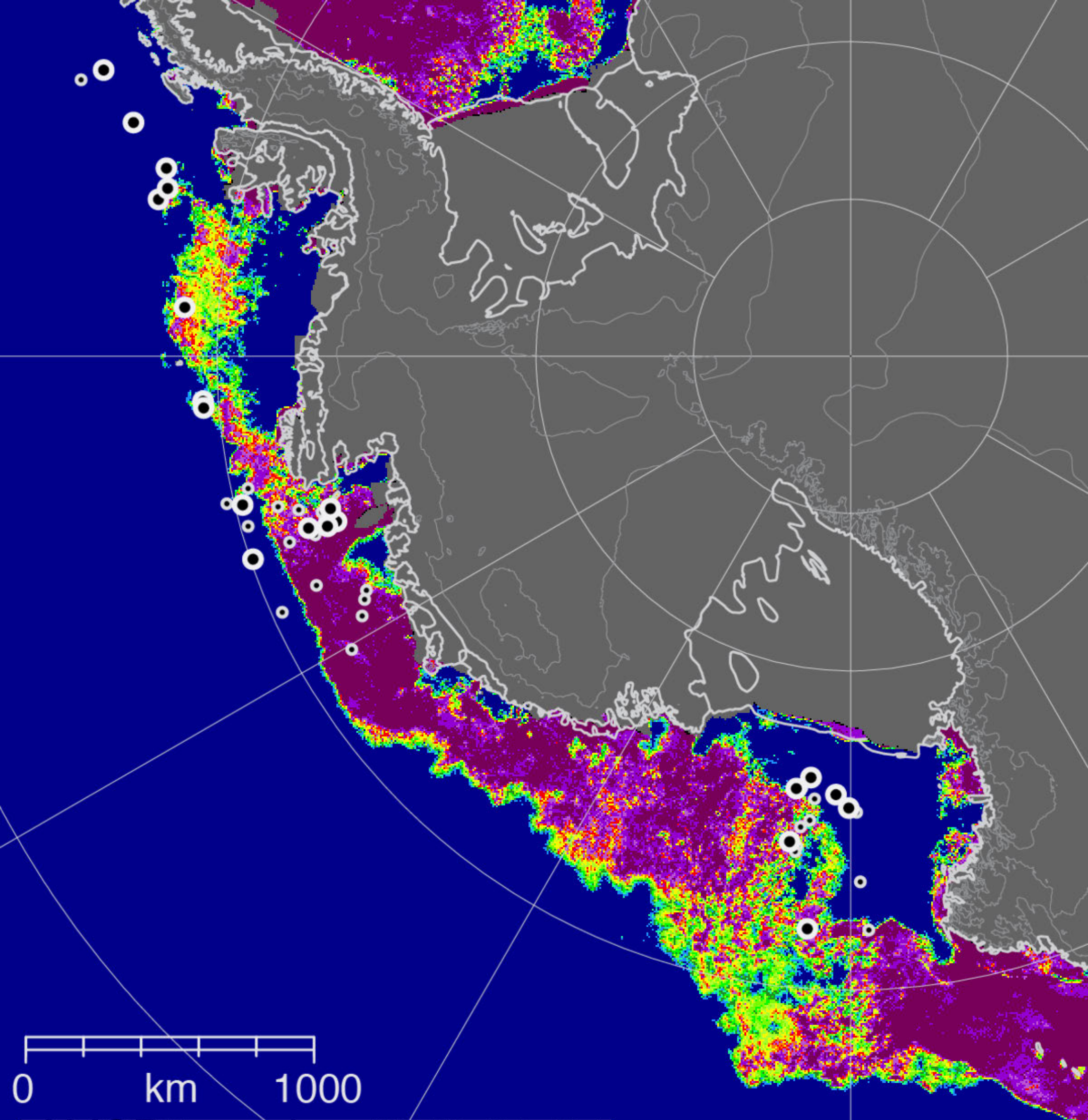
AMSR2 sea ice: 2013-01-07
