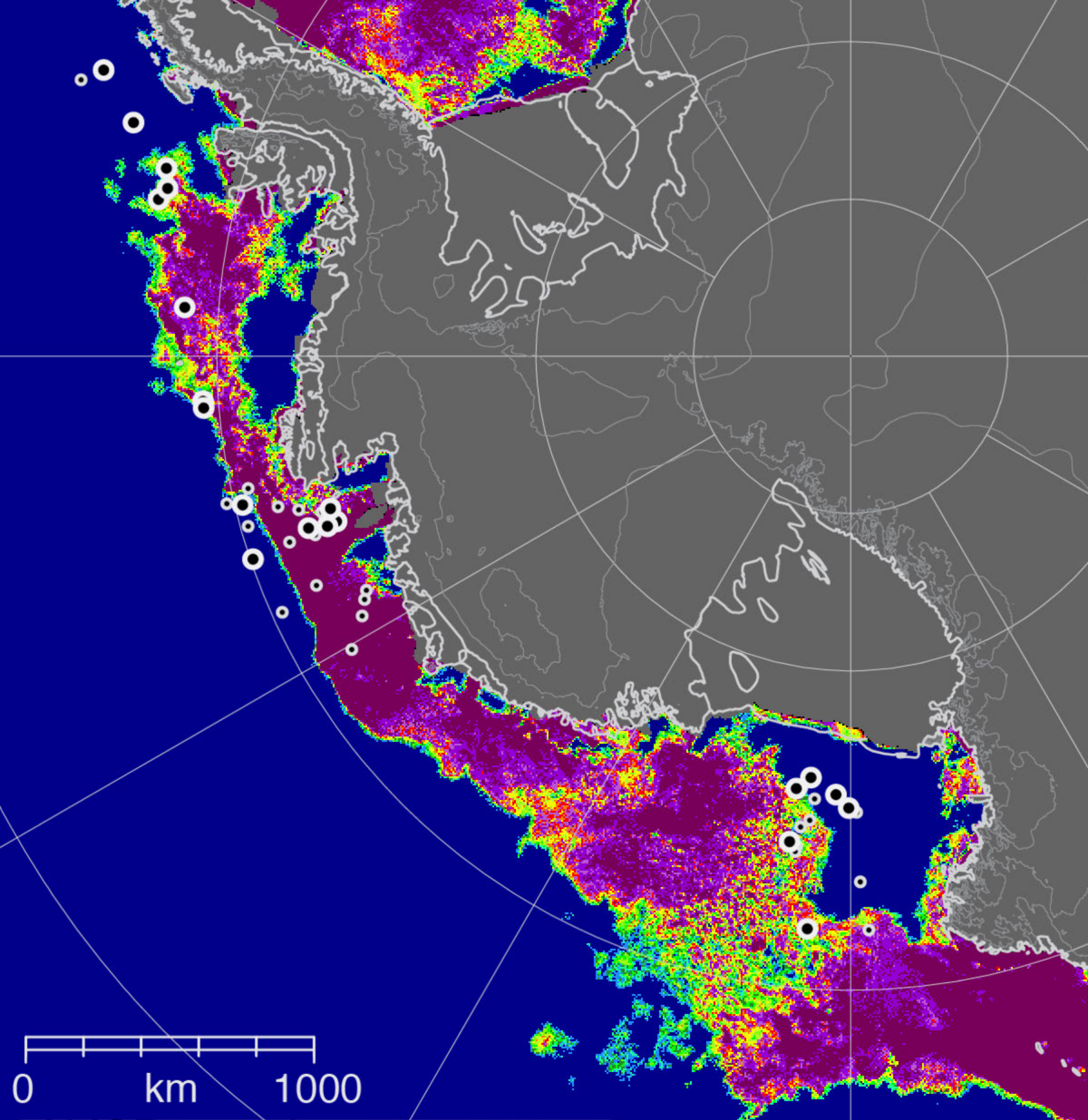
AMSR2 sea ice: 2012-12-31
