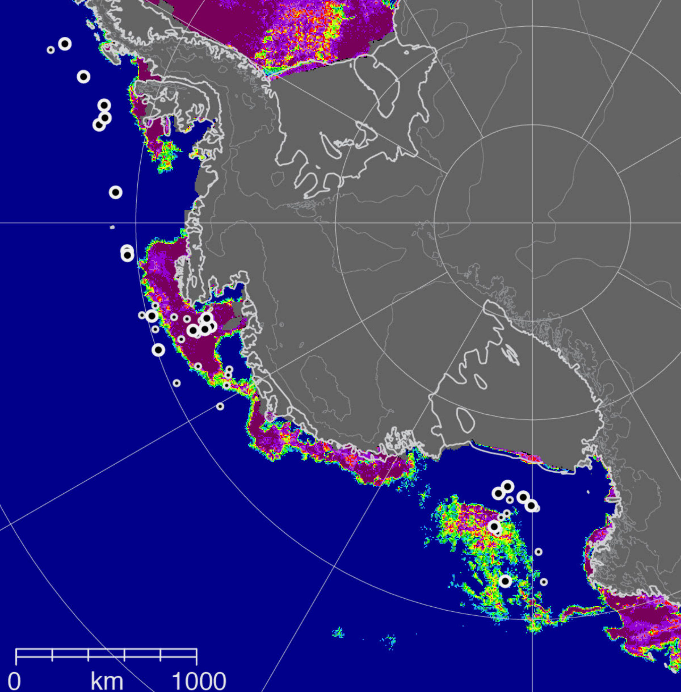
AMSR2 sea ice: 2015-02-09
