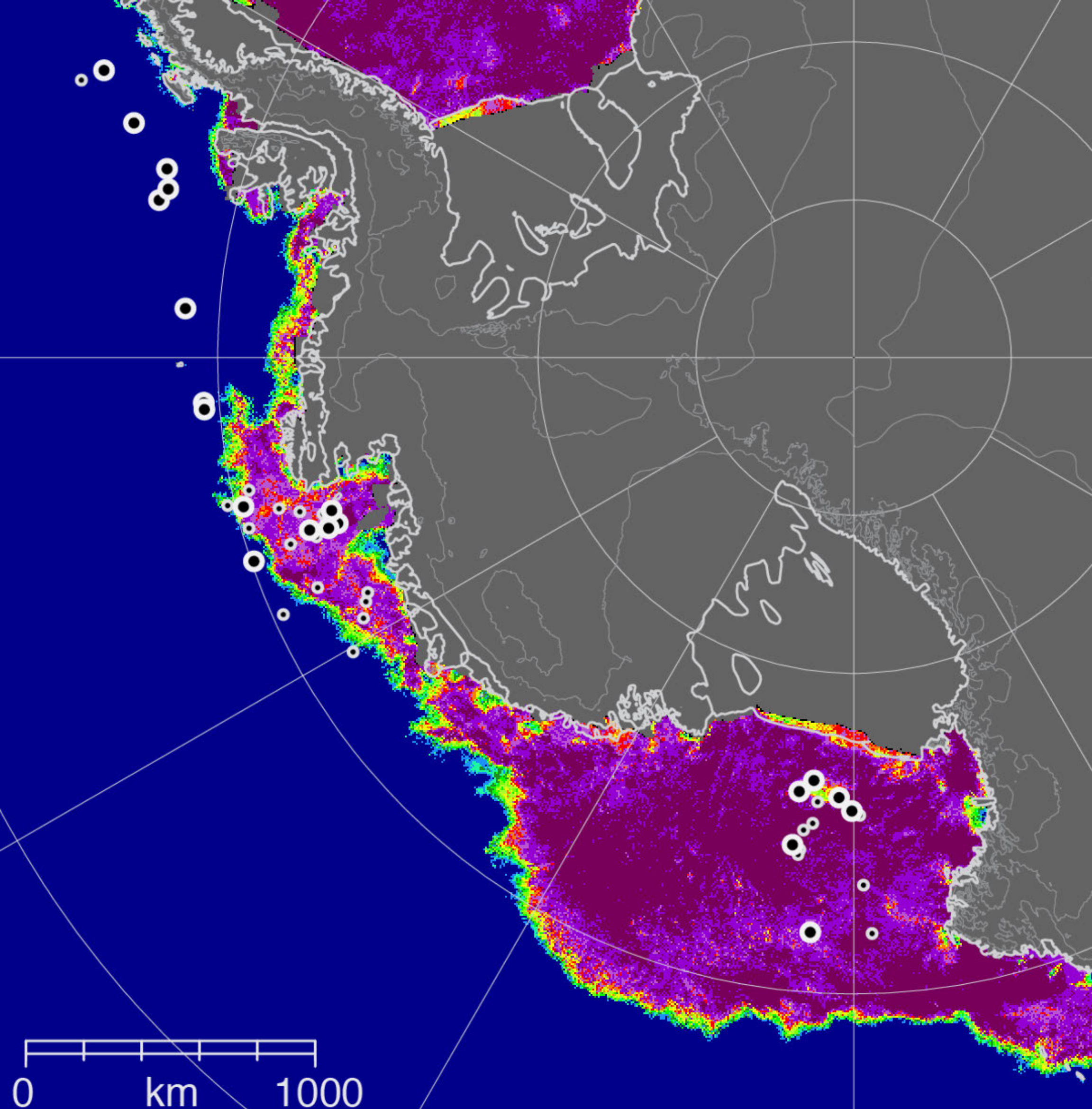
AMSR2 sea ice: 2015-03-30
