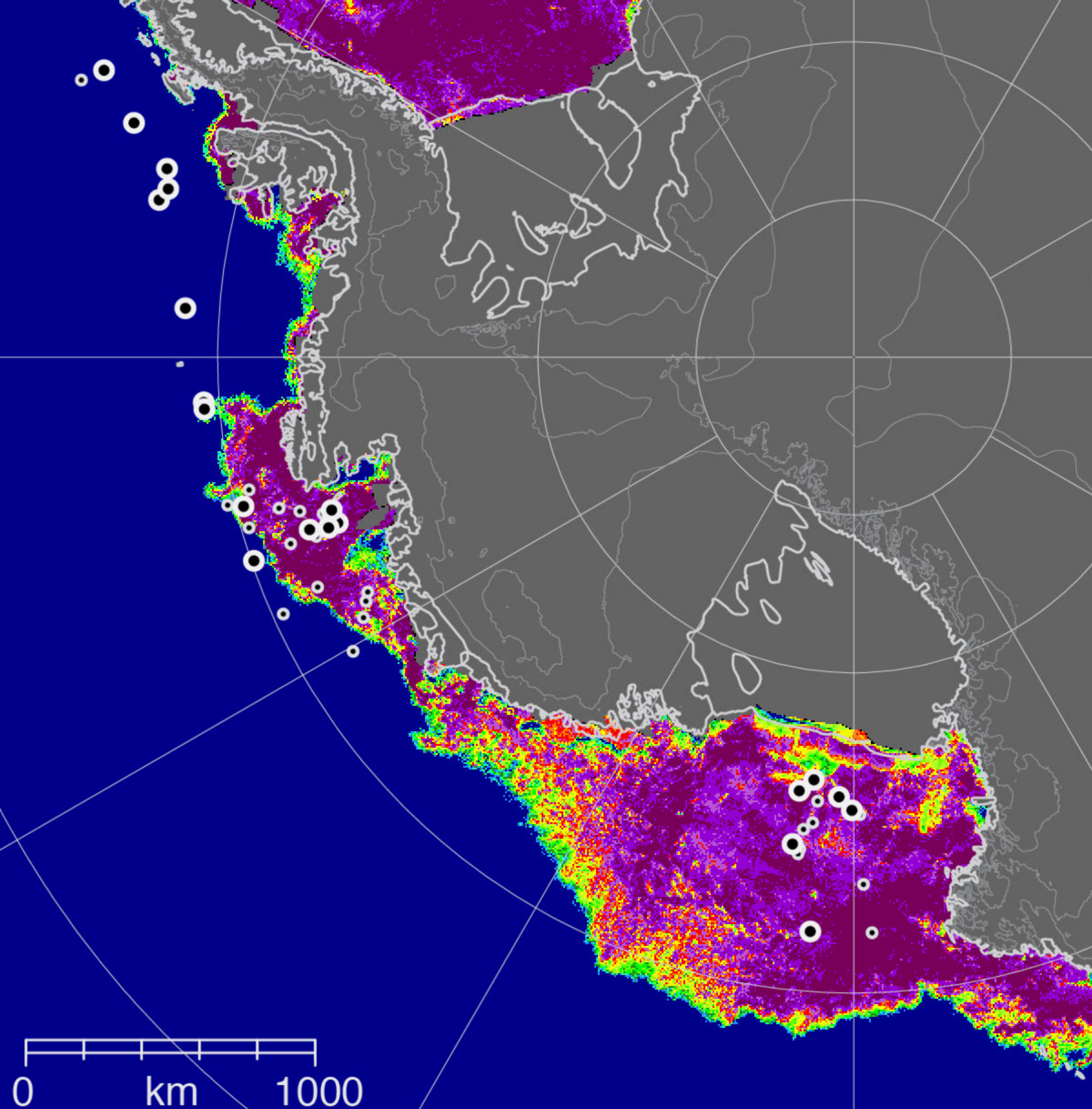
AMSR2 sea ice: 2015-03-23
